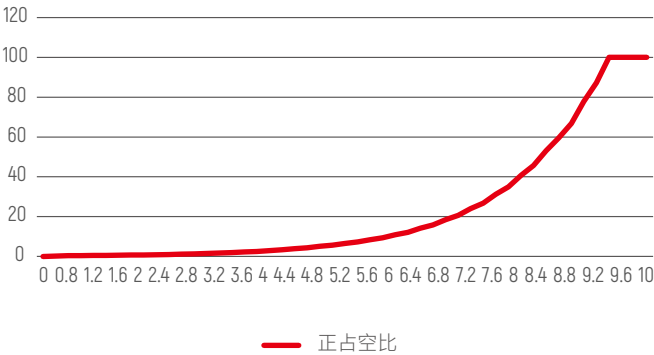
0/1-10V Curve
