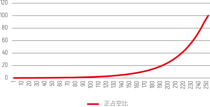
DALI Curve
