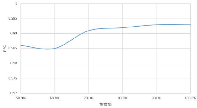
KVG-48600-DH PFC曲线
